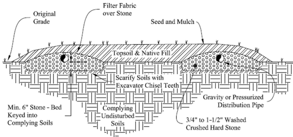
Cross-Section View
